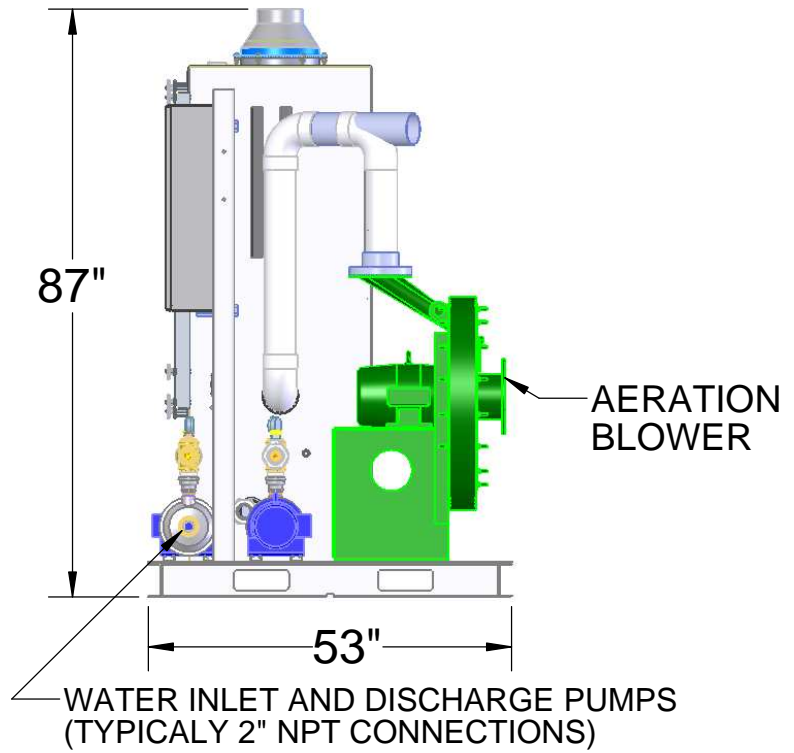
SIDE VIEW
